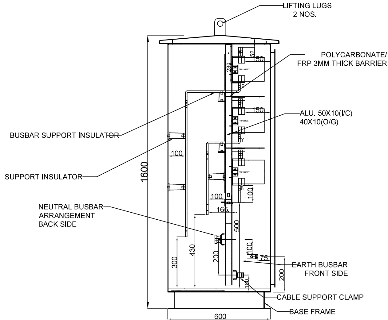
SIDE VIEW (INSIDE ARRANGEMENT)
