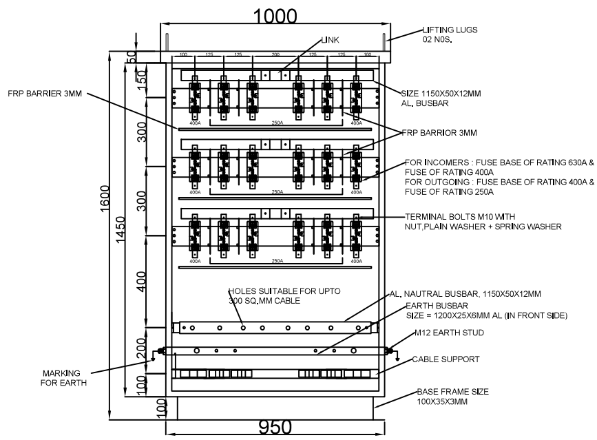
FRONT VIEW (INSIDE ARRANGEMENT)
