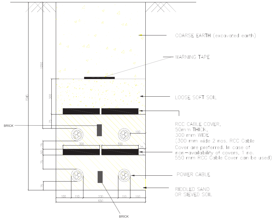
Figure 1.7 – 33kV Buried Cable Option-1 for Four Circuits
