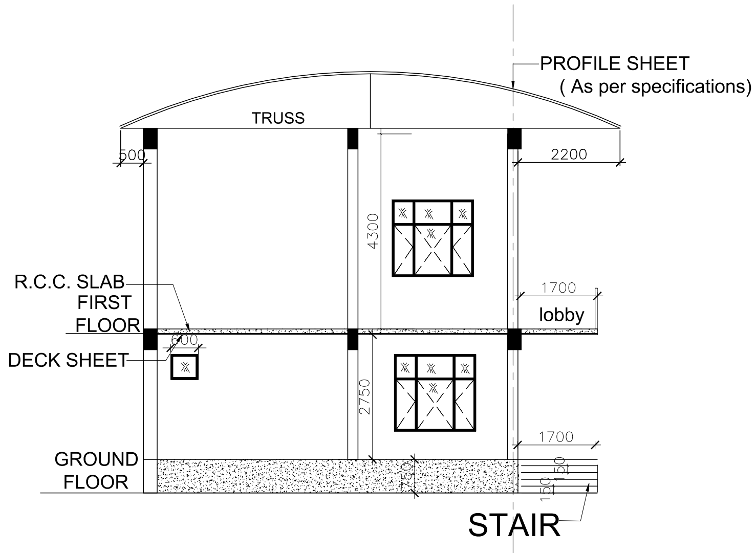
SIDE ELEVATION
