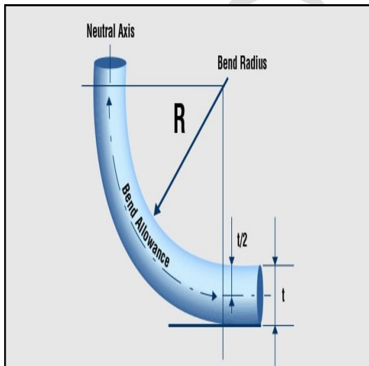
Figure 1: Min Bending Radius = OD × Bending Factor Figure 2
