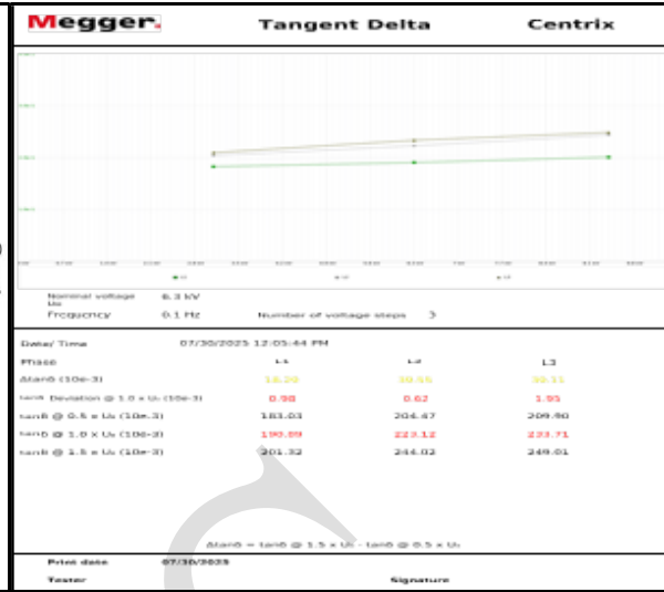
Figure 16(Tan)
