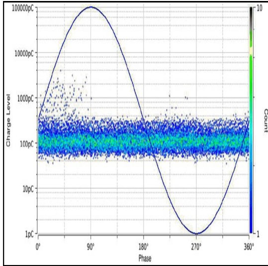
Figure 15(PRPD)
