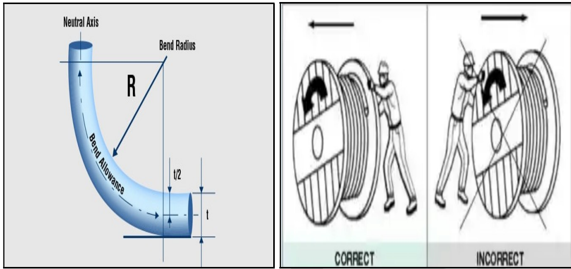
Figure 1: Min Bending Radius = OD × Bending Factor Figure 2
