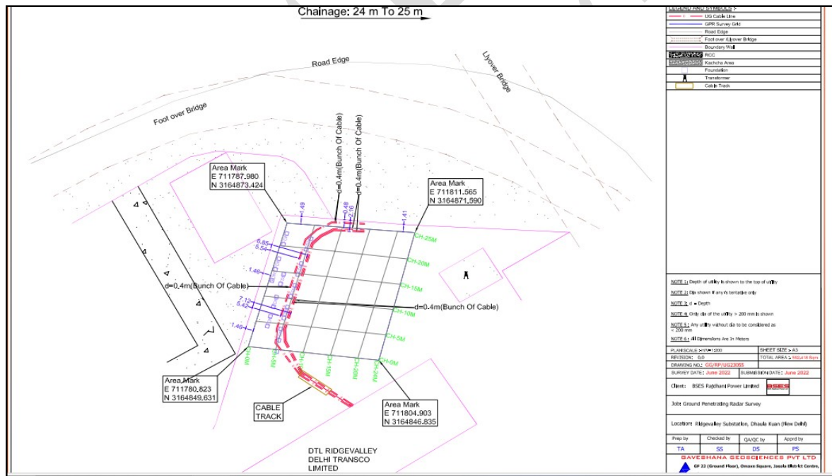
Figure 5 (GPR Map)
