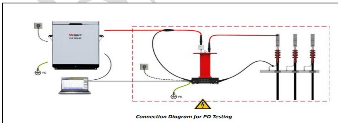
Figure 14(PD testing kit & connection details)
