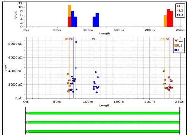
Figure 18(PD Mapping)
