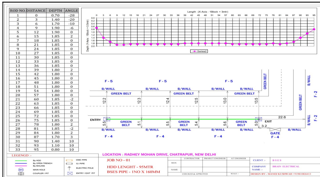
Figure 6 (Trenchless Map)
