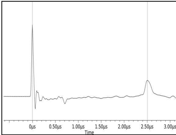
Figure 17(PD Calibration)
