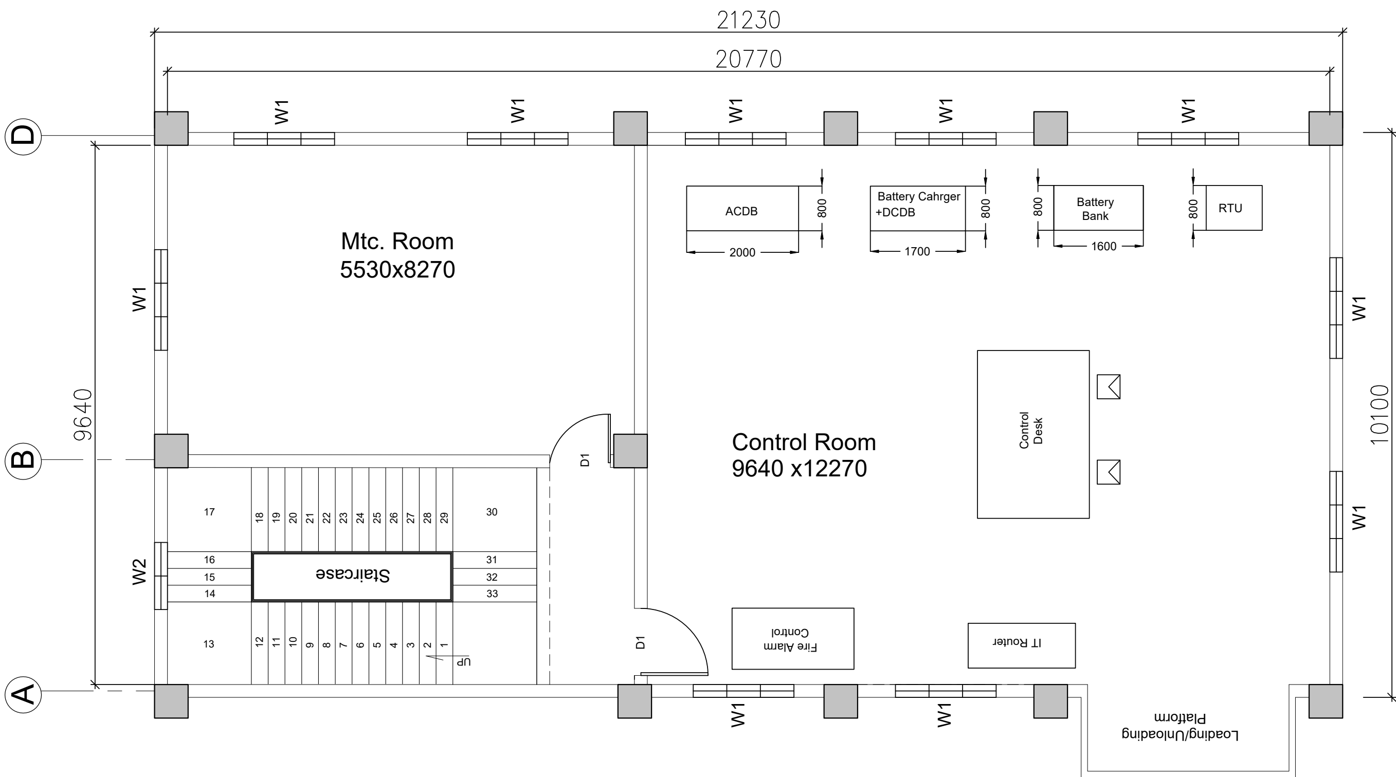
LAYOUT PLAN - FIRST FLOOR (DTC DEPOT AT PREERAGARHI)
