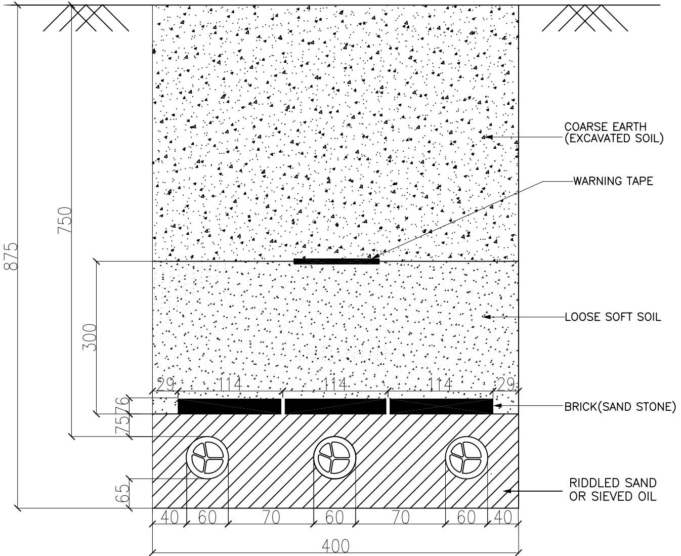
TYPICAL DETAILS FOR 1.1KV BURRIED CABLE TYPE – A 1
